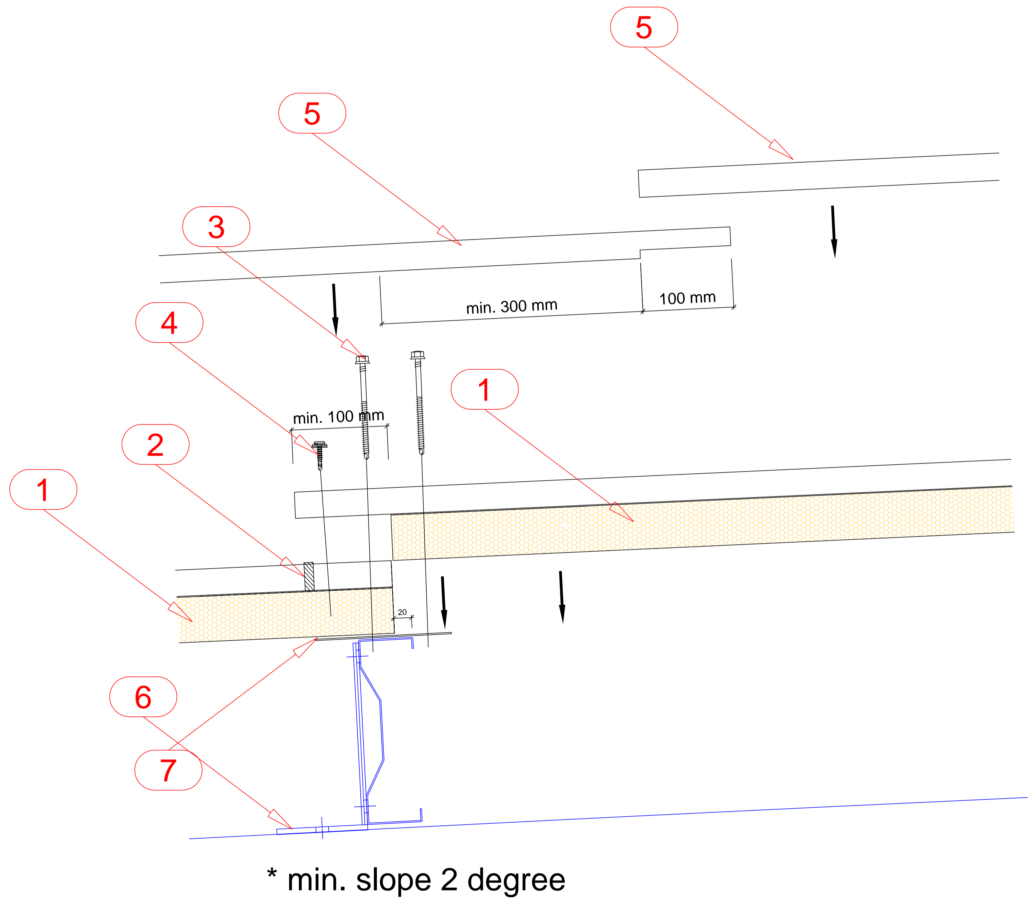
B Joint Detail Scale 1/10
