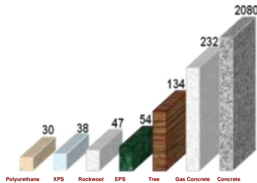
Insulation Efficiency of Building Materials
